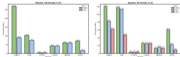
Figure 4: Throughput comparison of various plotters
