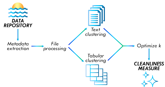
Figure 1: Clustering pipeline.
